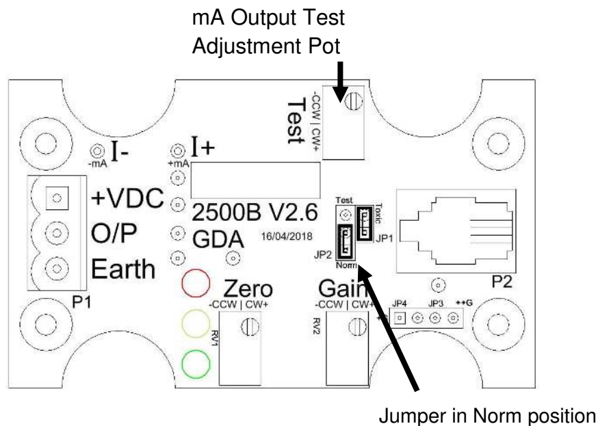
Figure 8: JP2 Jumper in Normal operation
